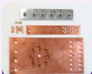
Bolted and Clinched Bus Bars
